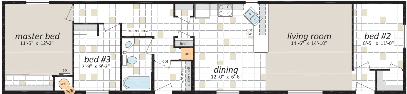
PR-1054, 16' x 68', 3FB-1B
